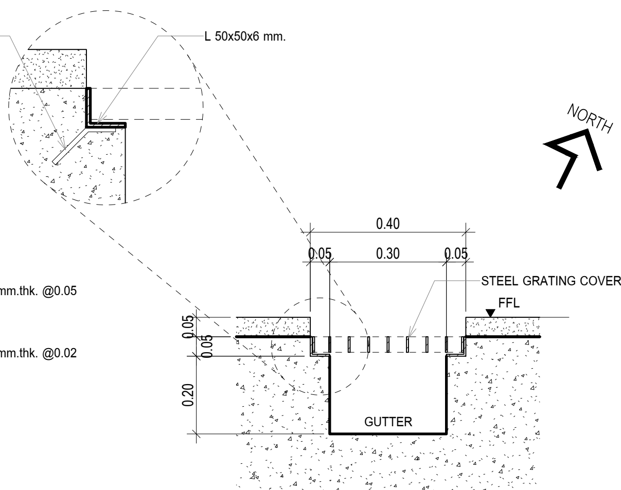
SECTION B
