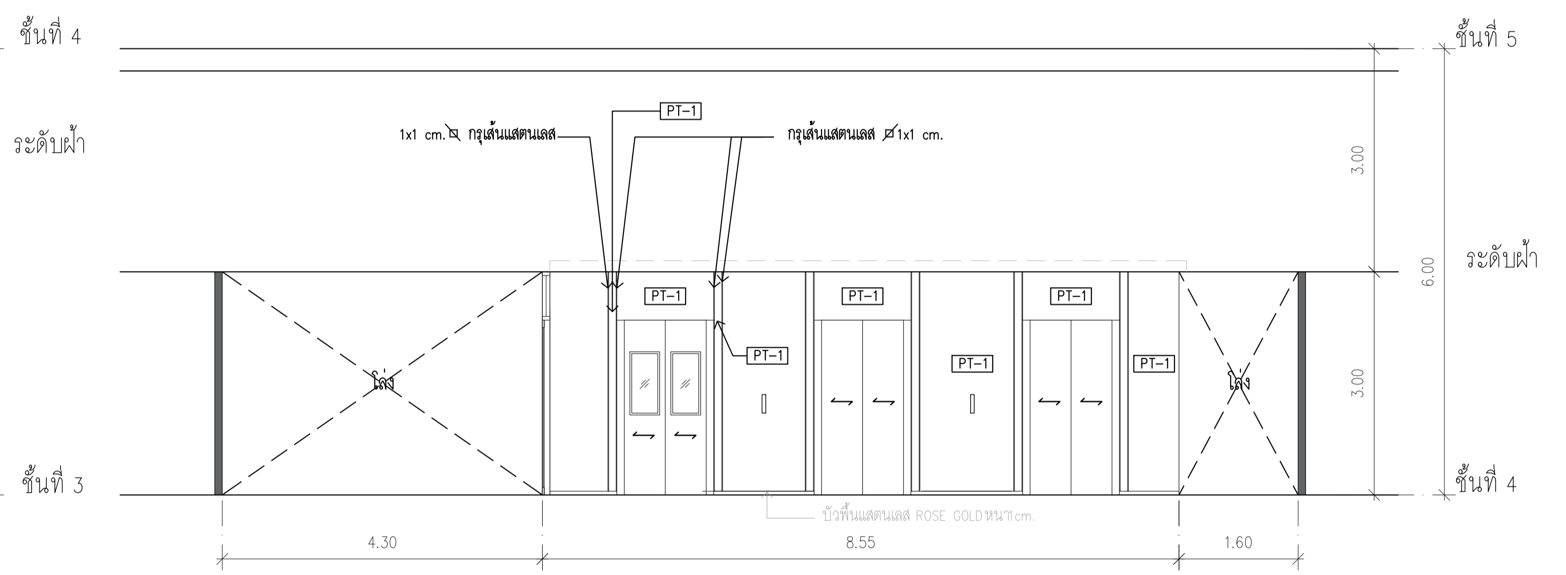
4th FLOOR ELEVATION 2 SCALE 1:50
