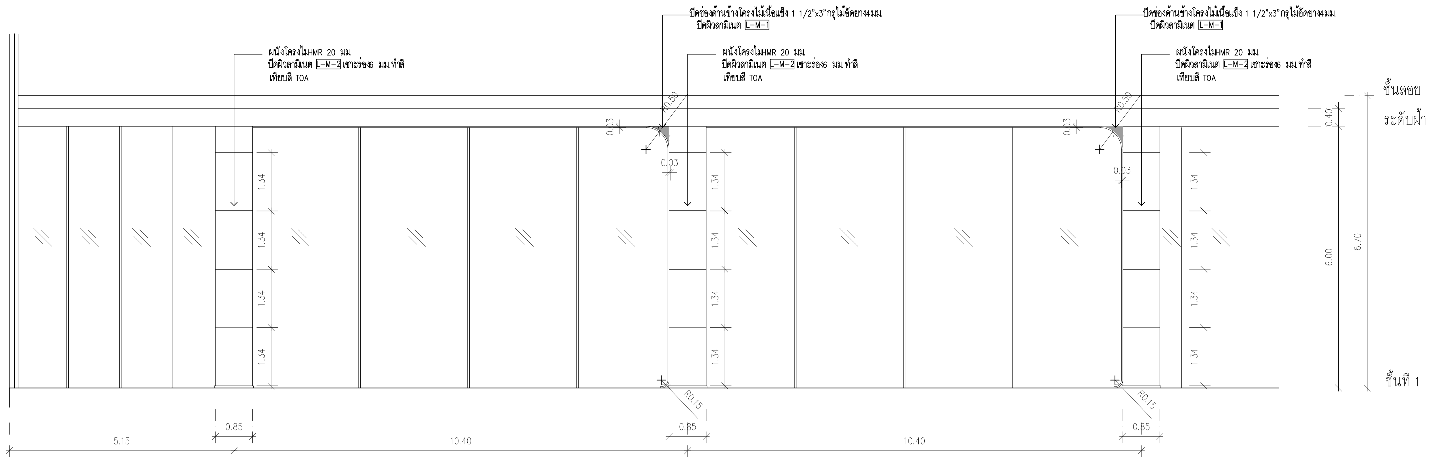
GROUND FLOOR ELEVATION 4 SCALE 1:50
