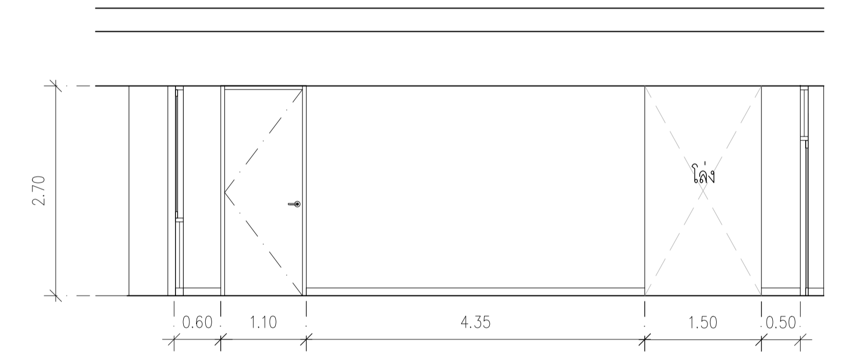
23rd Floor ELEVATION 5 SCALE 1:50
