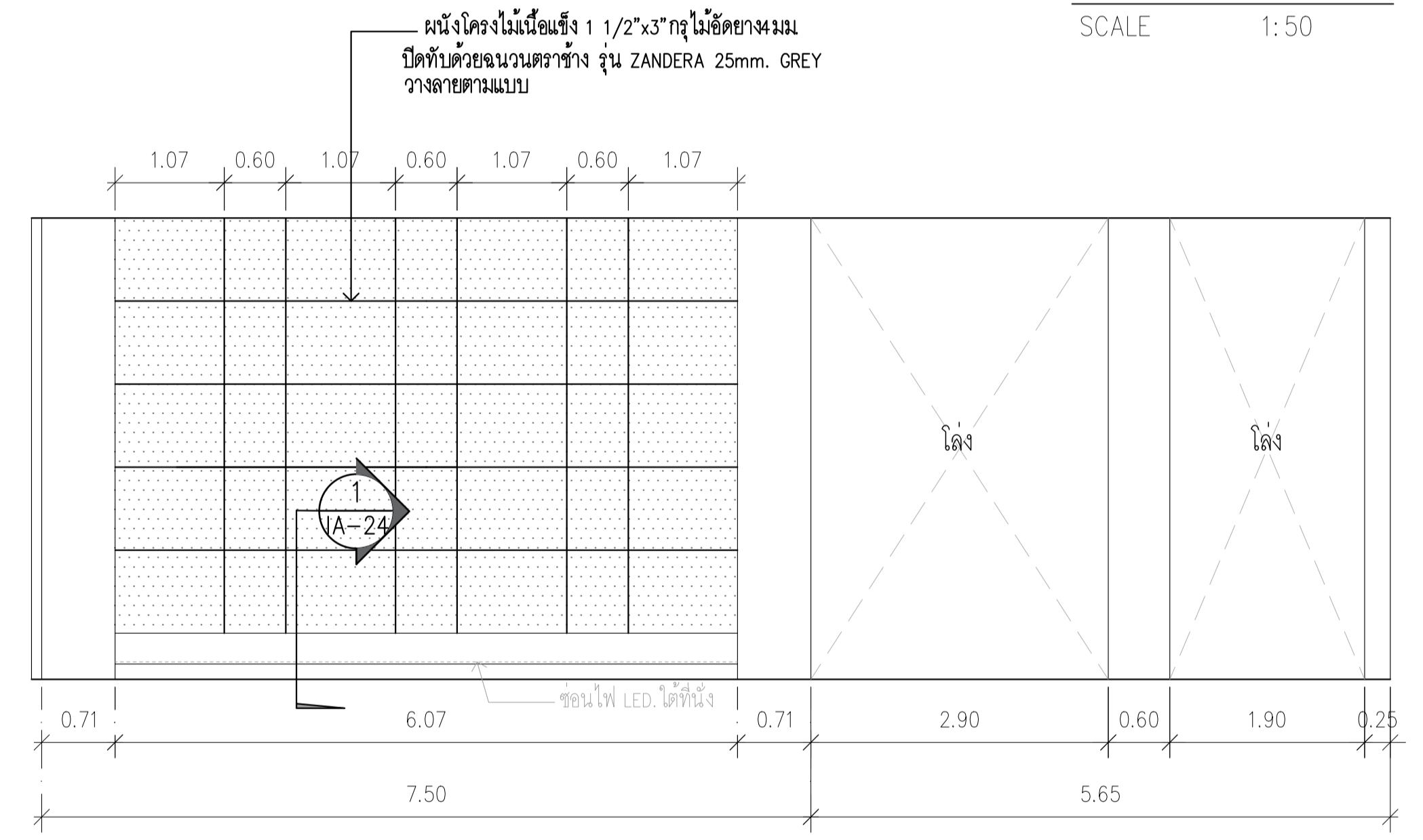
ELEVATION 2 SCALE 1:50
