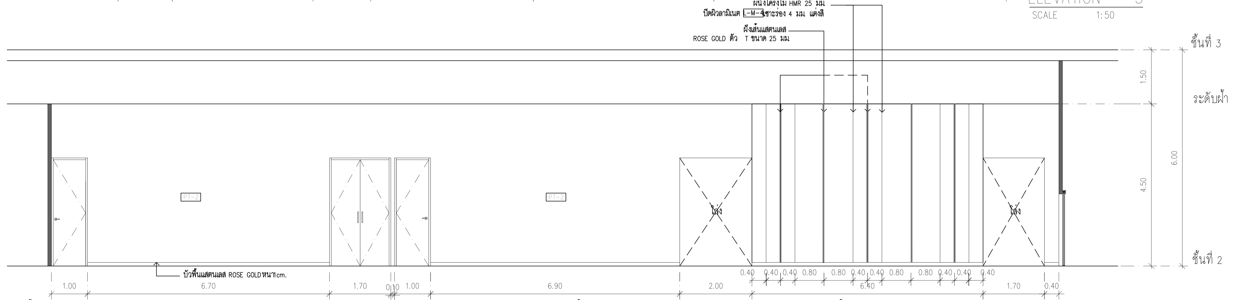
ELEVATION 4 SCALE 1:50
