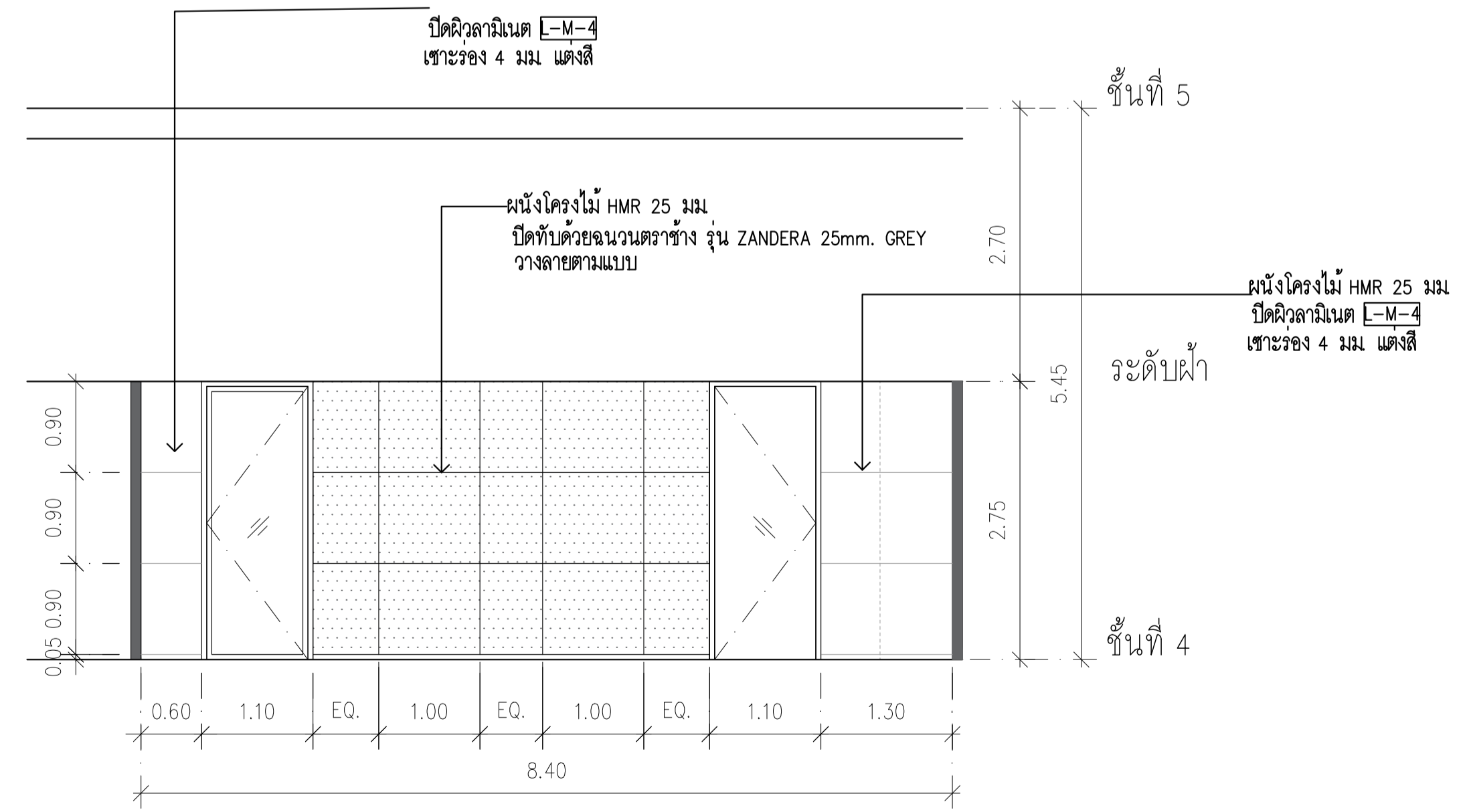
ELEVATION 2 SCALE 1:50 CLASSROOM S
