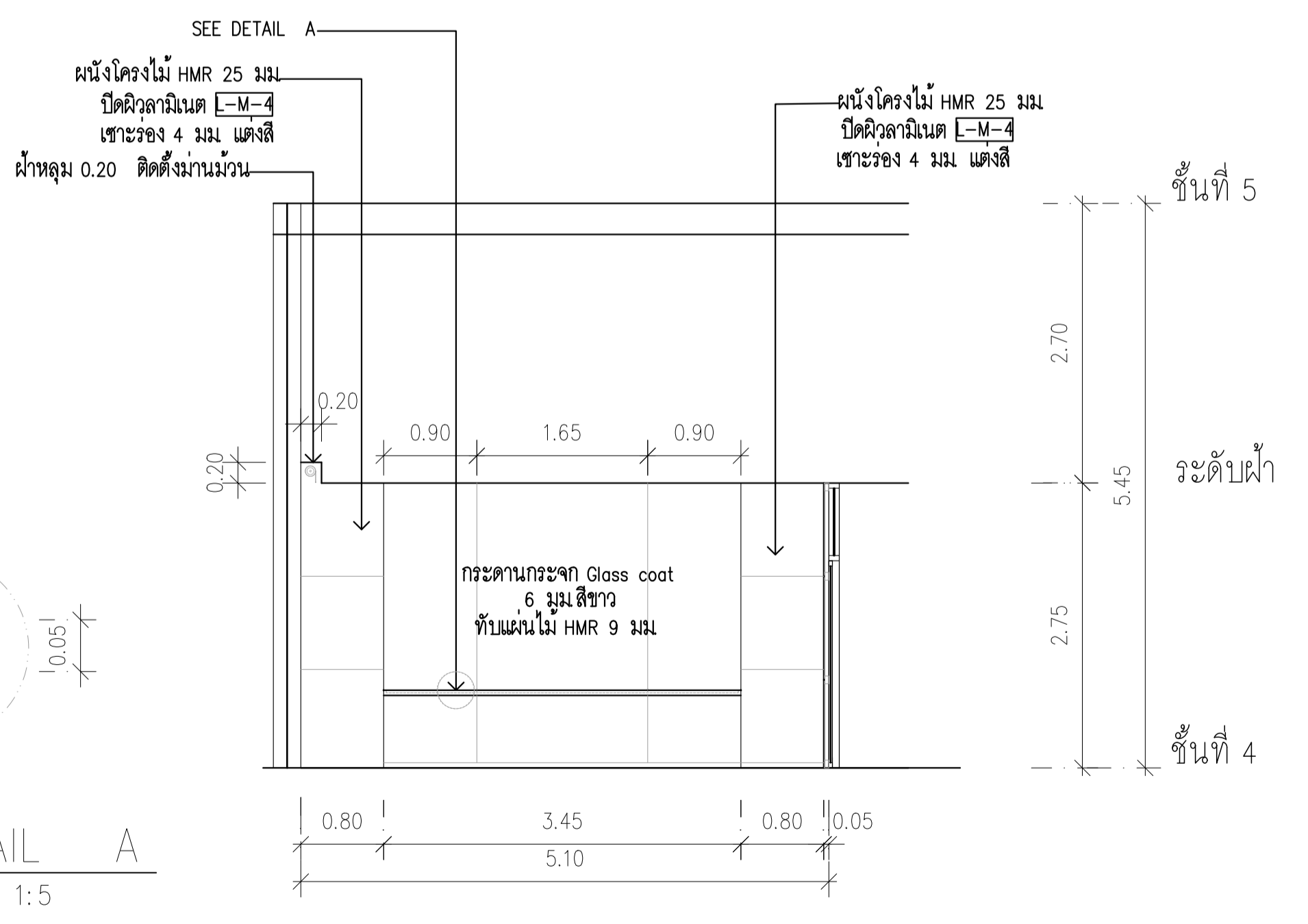
ELEVATION 1 SCALE 1:50
