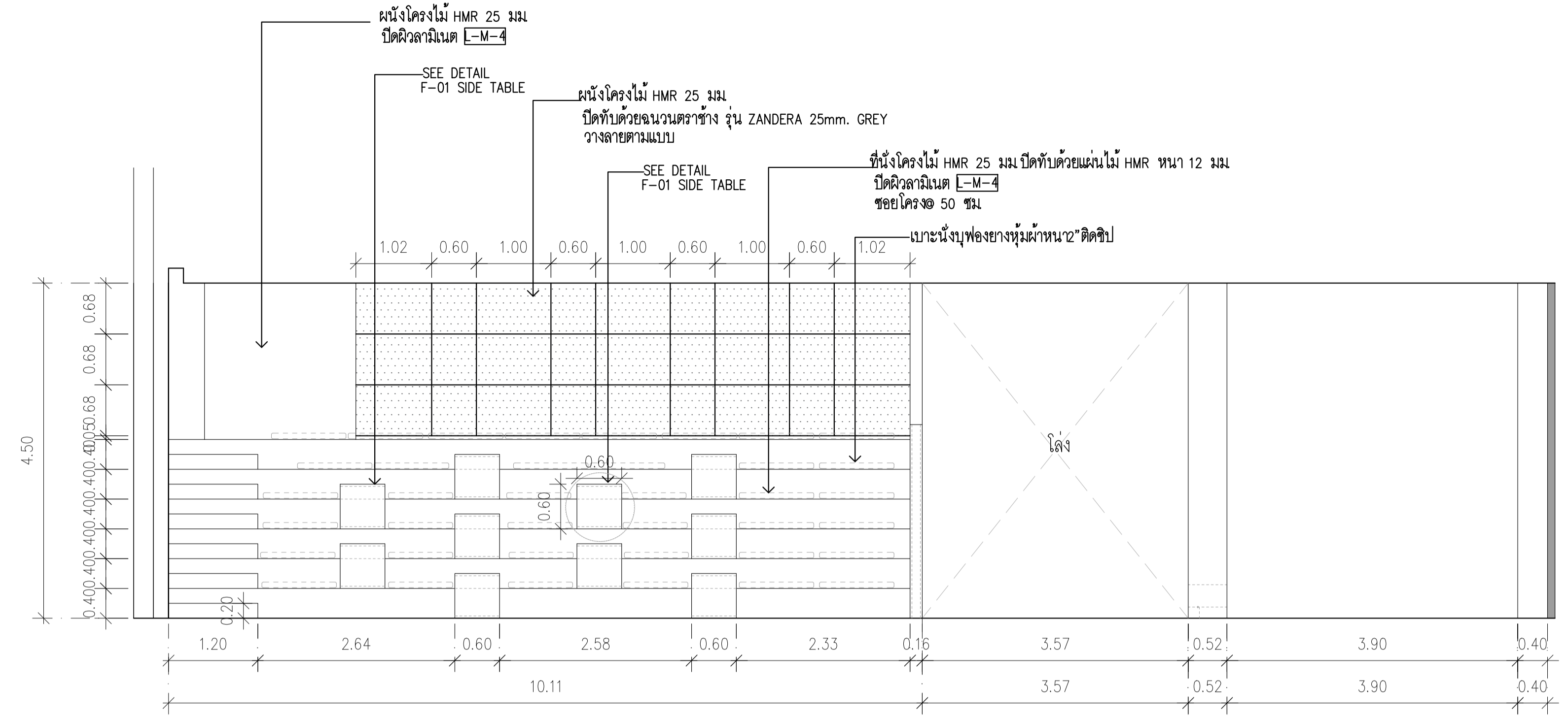
ELEVATION 1 SCALE 1:50
