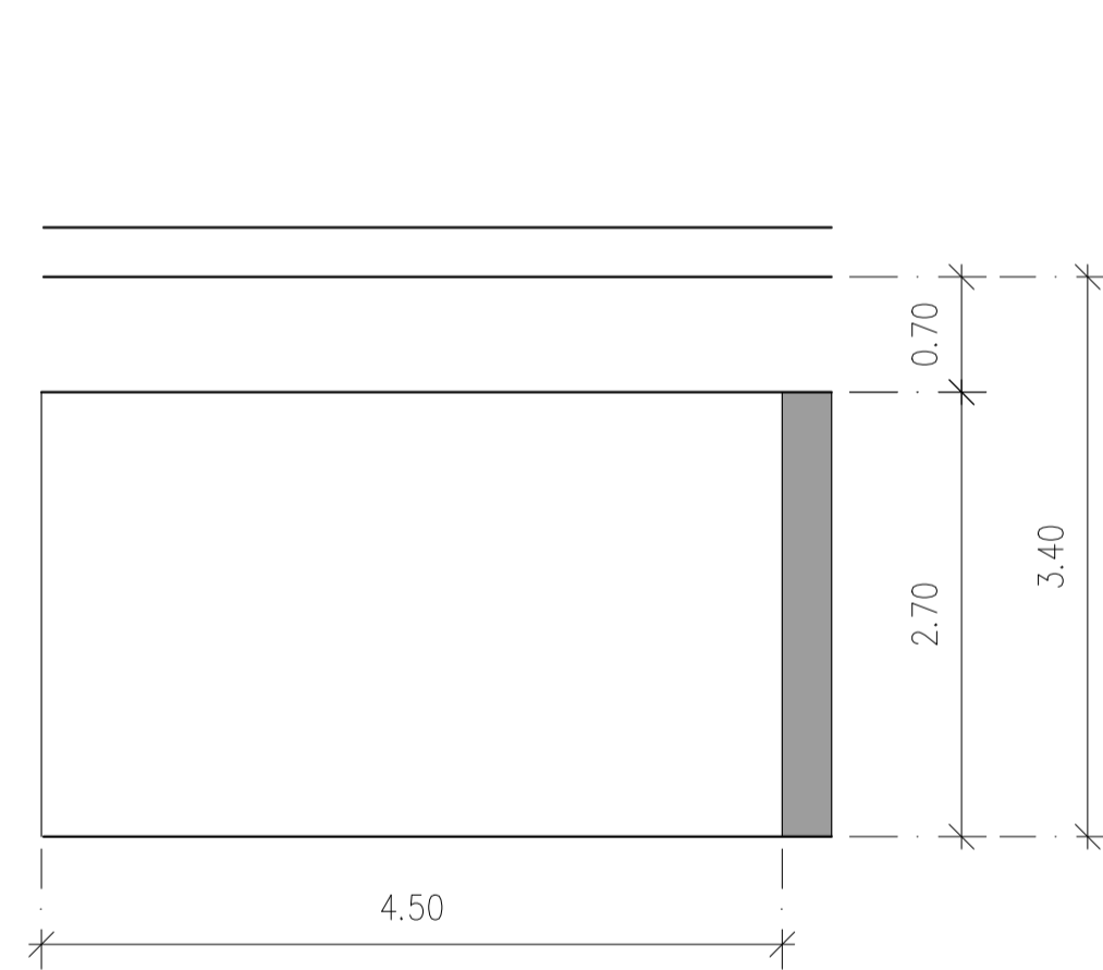
14th-22th Floor ELEVATION 3 SCALE 1:50
