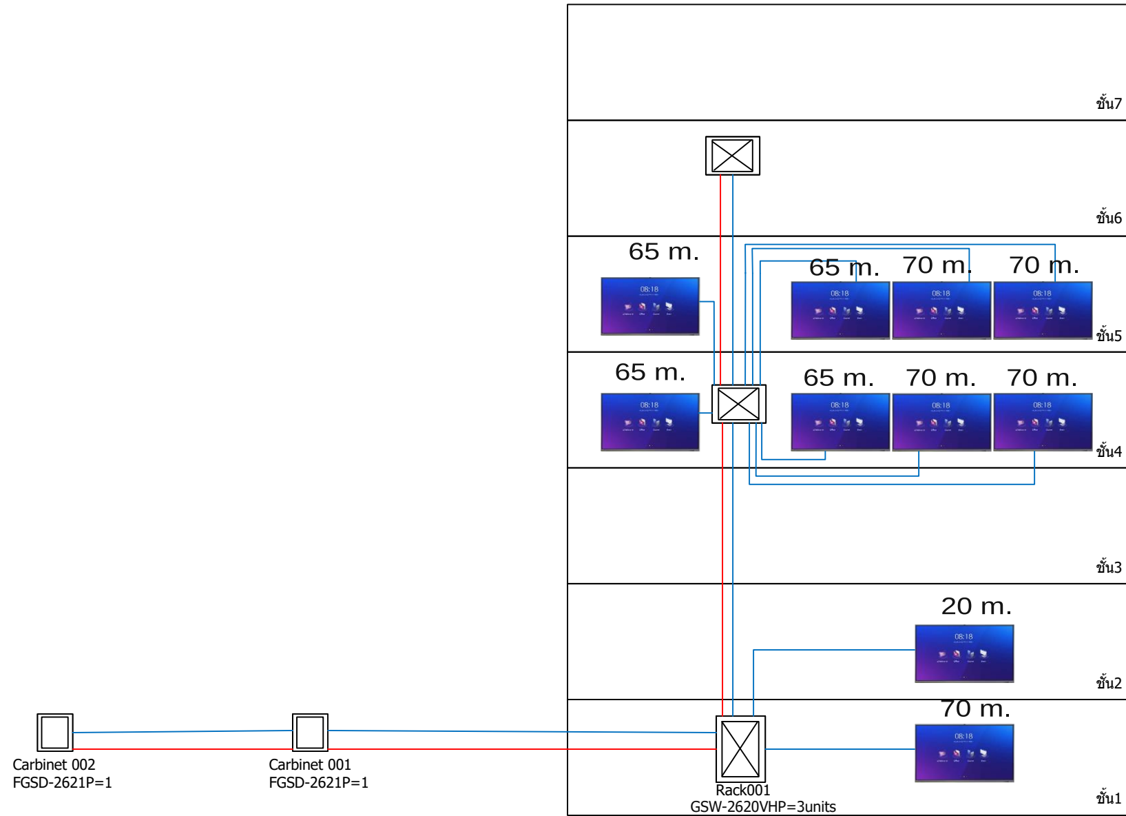
Rack27U + Switch
