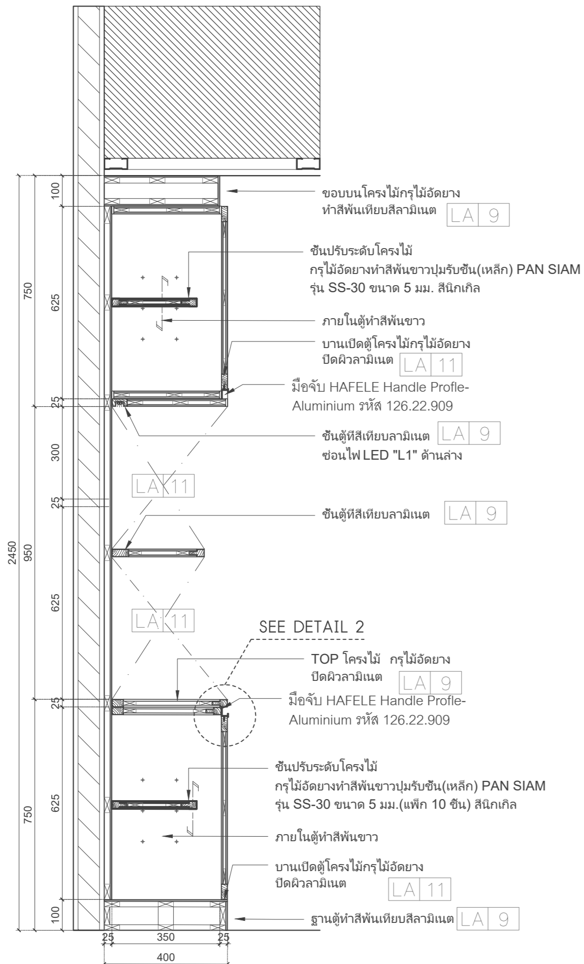
1 SECTION 3 SCALE 1 : 12.5
