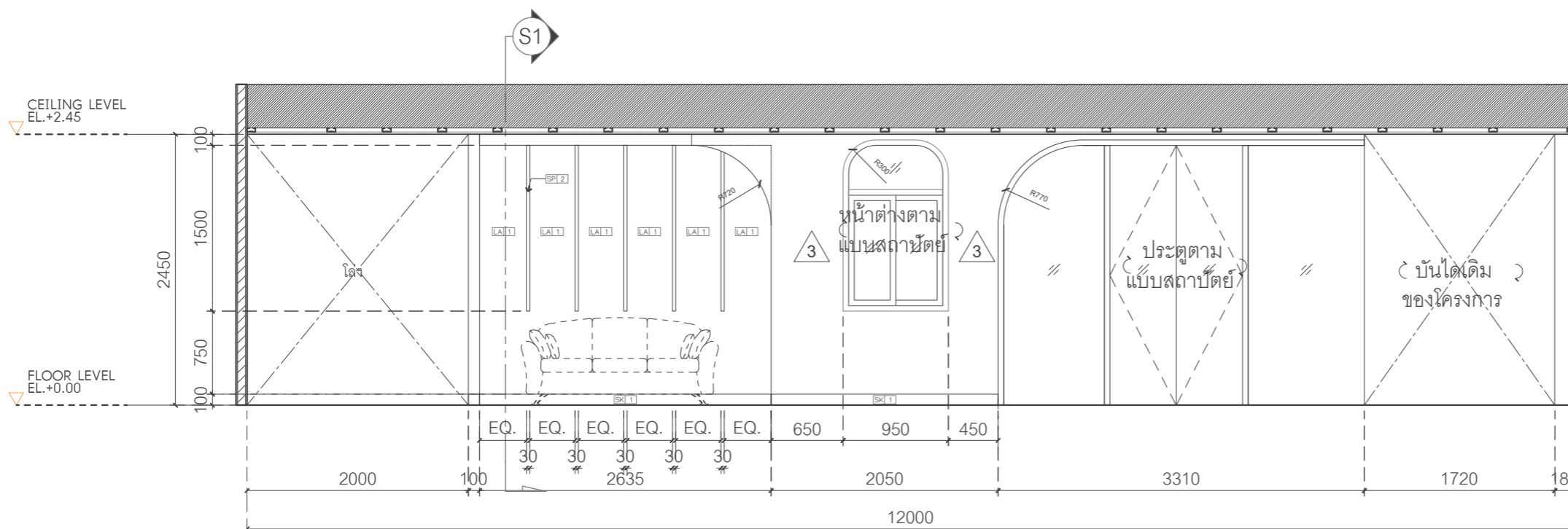
2 ELEVATION-E1 SCALE 1 : 50
