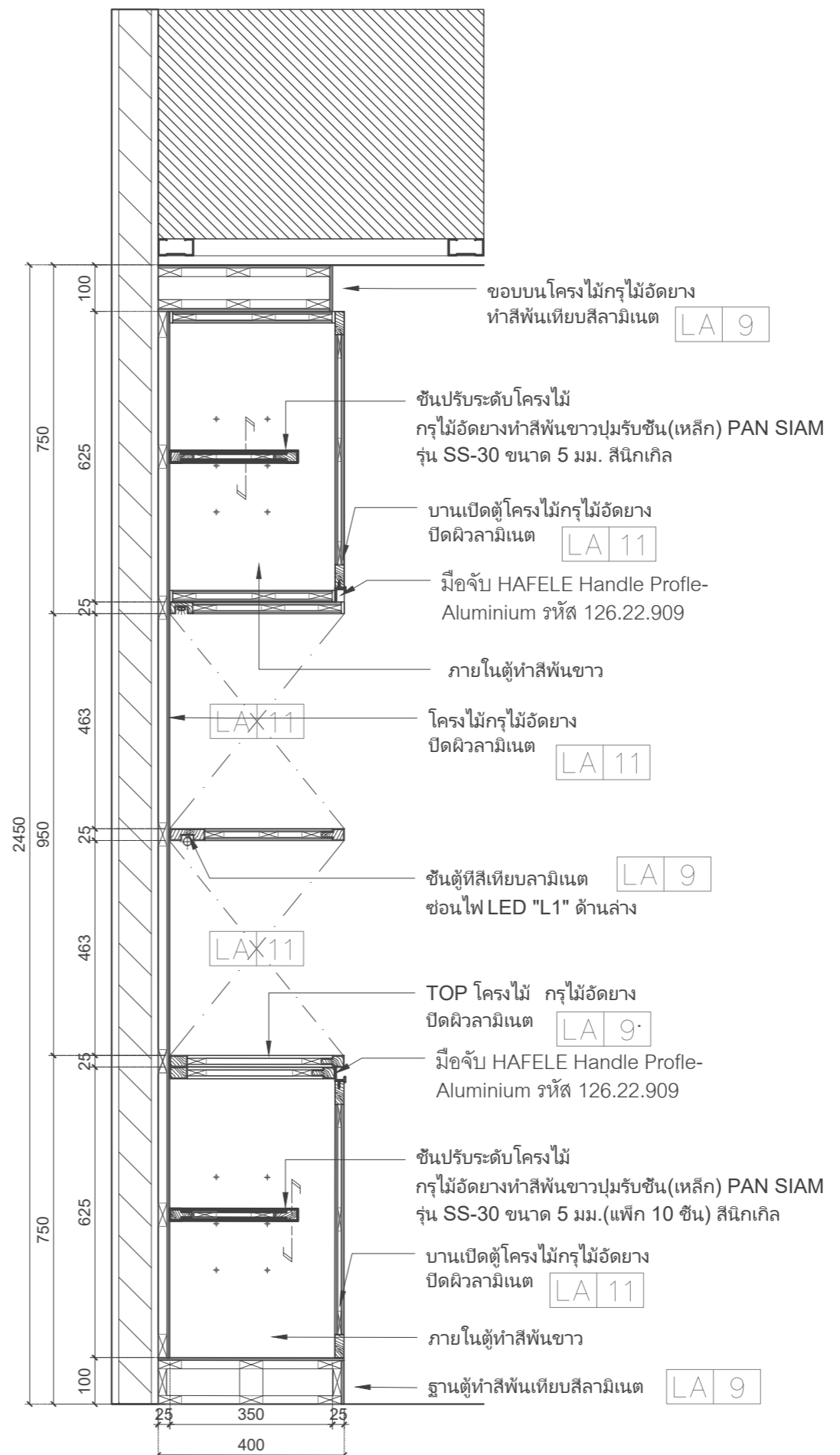
2 SECTION 4 SCALE 1 : 12.5
