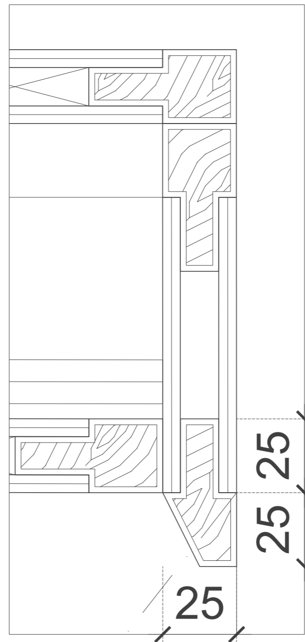
○ CELING DETAIL 3 SCALE 1 : 5
