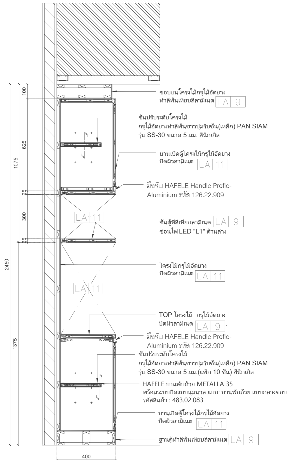
2 SECTION 2 SCALE 1 : 12.5
