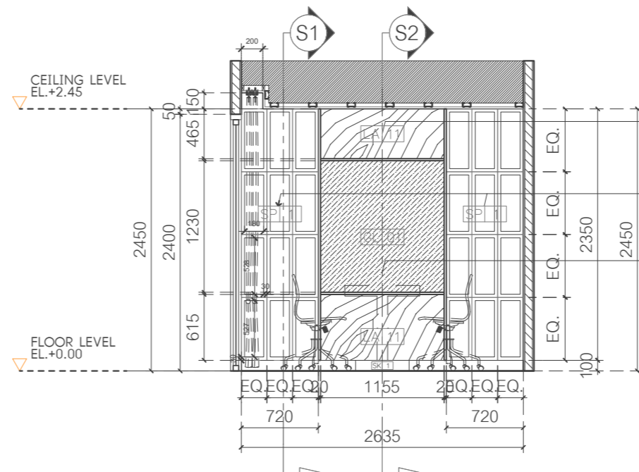
2 ELEVATION-E1 SCALE 1 : 50
