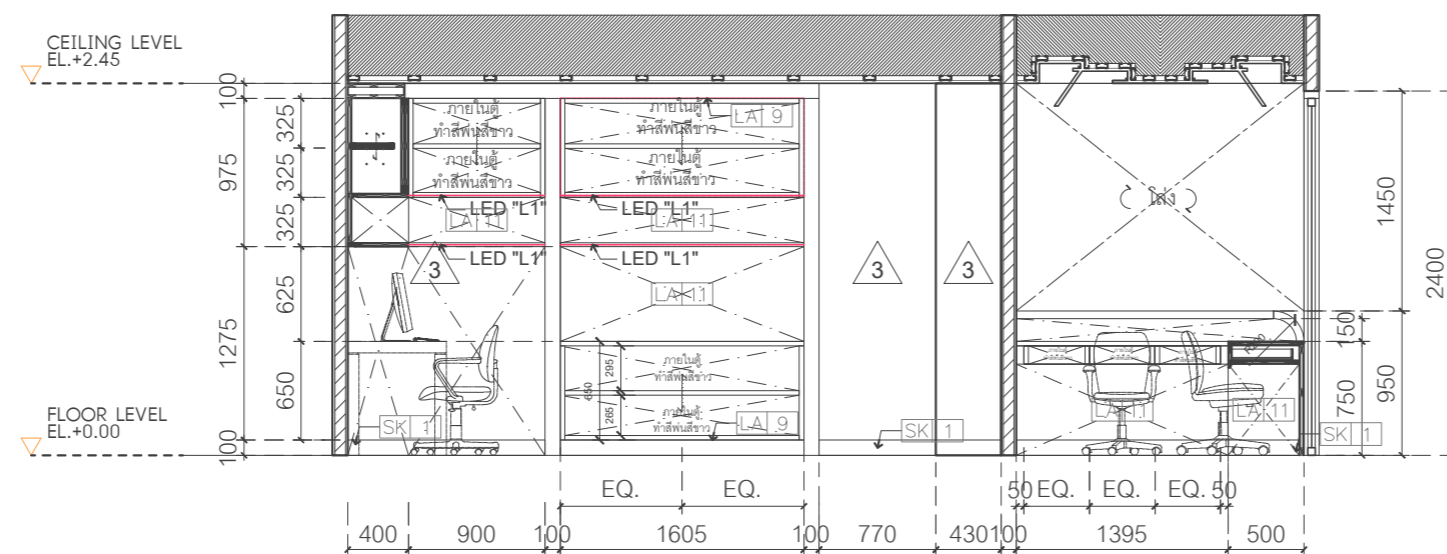
2 INSIDE ELEVATION-E3 SCALE 1 : 50
