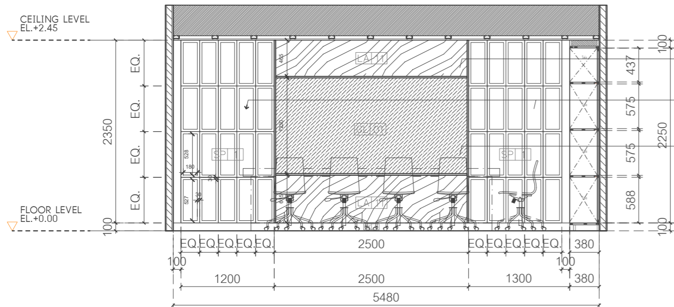
3 ELEVATION-E2 SCALE 1 : 50
