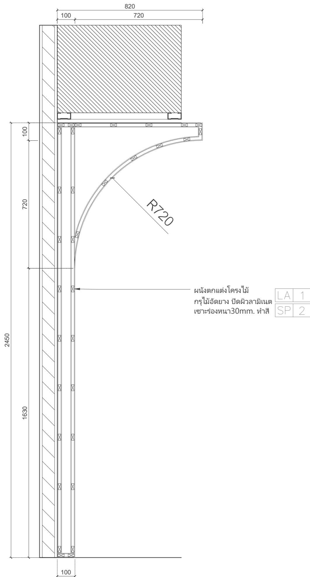
1 SECTION 1 SCALE 1 : 12.5
