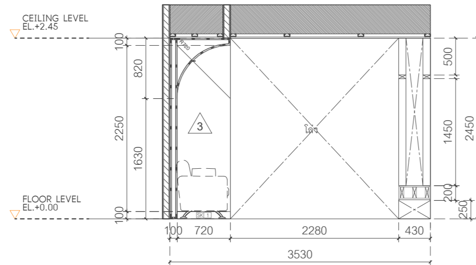
1 ELEVATION-E2 SCALE 1 : 50
