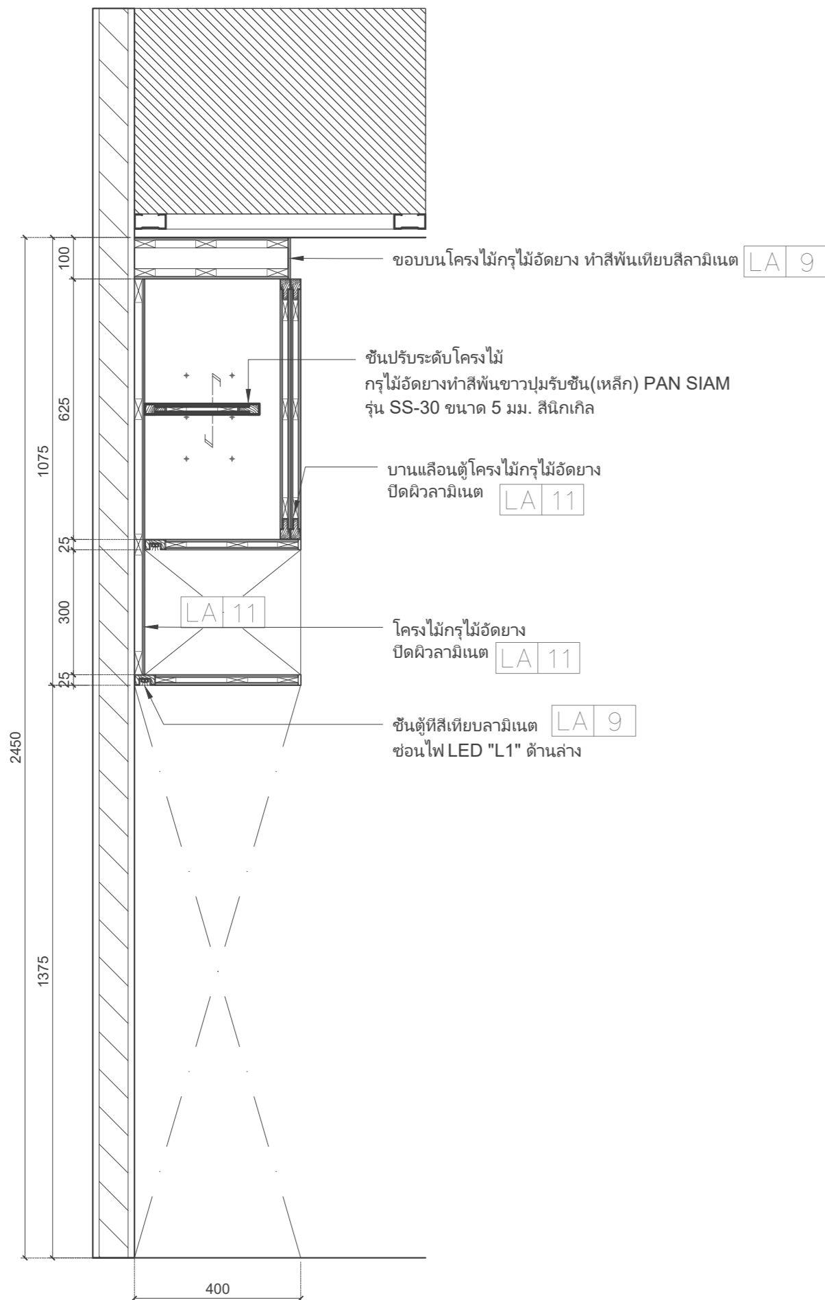
1 SECTION 1 SCALE 1 : 12.5
