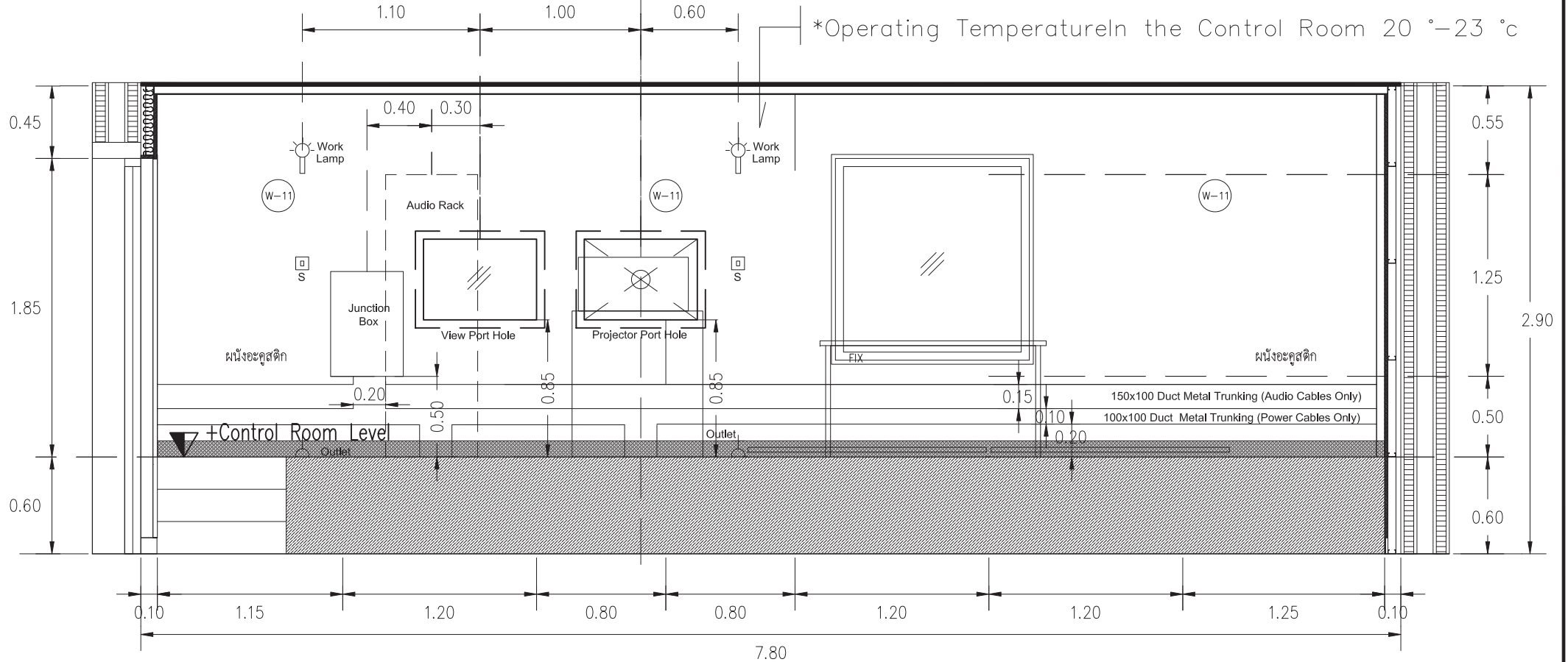
Detail Equipment Position Elevation for Control Room of Cosci Auditorium
