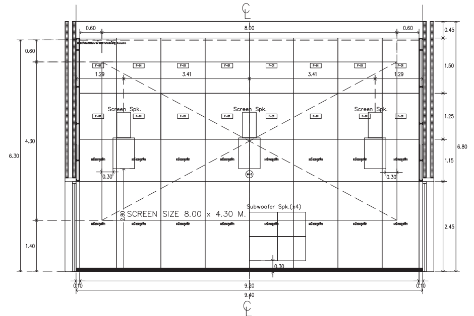
4 FRONT ELEVATION ELE. SCALE 1: 75
