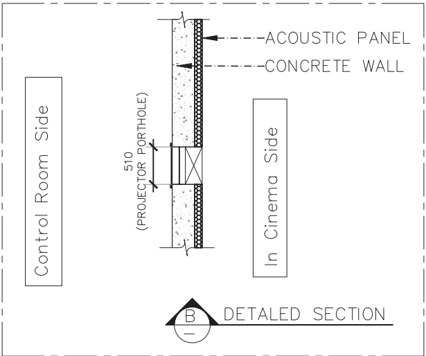
DETAIL DETAILED PROJECTION PORT HOLE AND VIEWING PORT HOLE
