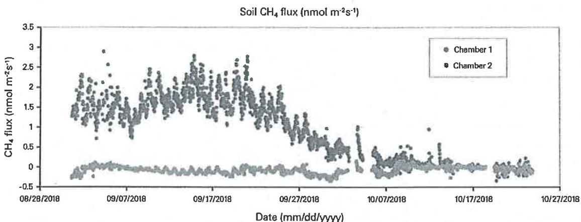
Figure 3. Seasonal soil \text{CH}_4 flux variations observed using the LI-7810 \text{CH}_4/\text{CO}_2/\text{H}_2\text{O} Trace Gas Analyzer and the LI-8150 Multiplexer with 8100-104 Long-Term Chambers. Chamber 1 site was a source of emissions up to 2.8 \text{ nmol m}^{-2}\text{s}^{-1} —which was unexpected for grassland. By October, the site had become a sink. Chamber 2 site was typically a sink with rates \sim -0.2 \text{ nmol m}^{-2}\text{s}^{-1} . This was expected and consistent with published rates.
