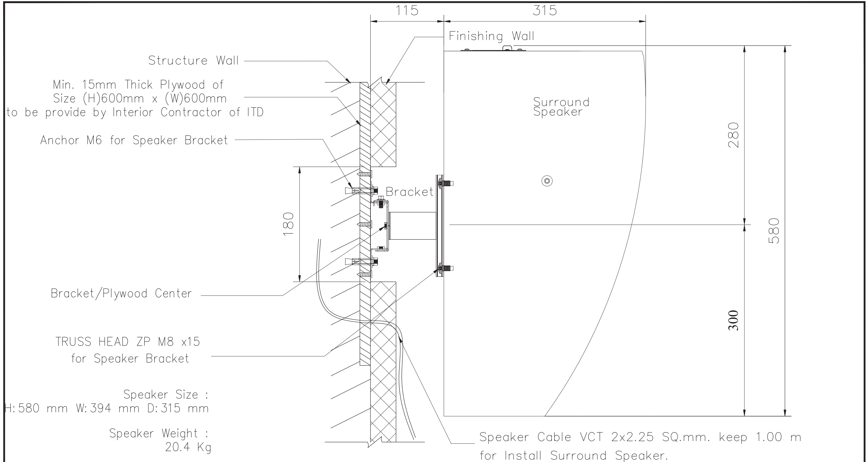
DETAIL 4 Detail Section of Surround Speaker Mounting for Cinema Size M (2nd Floor)
