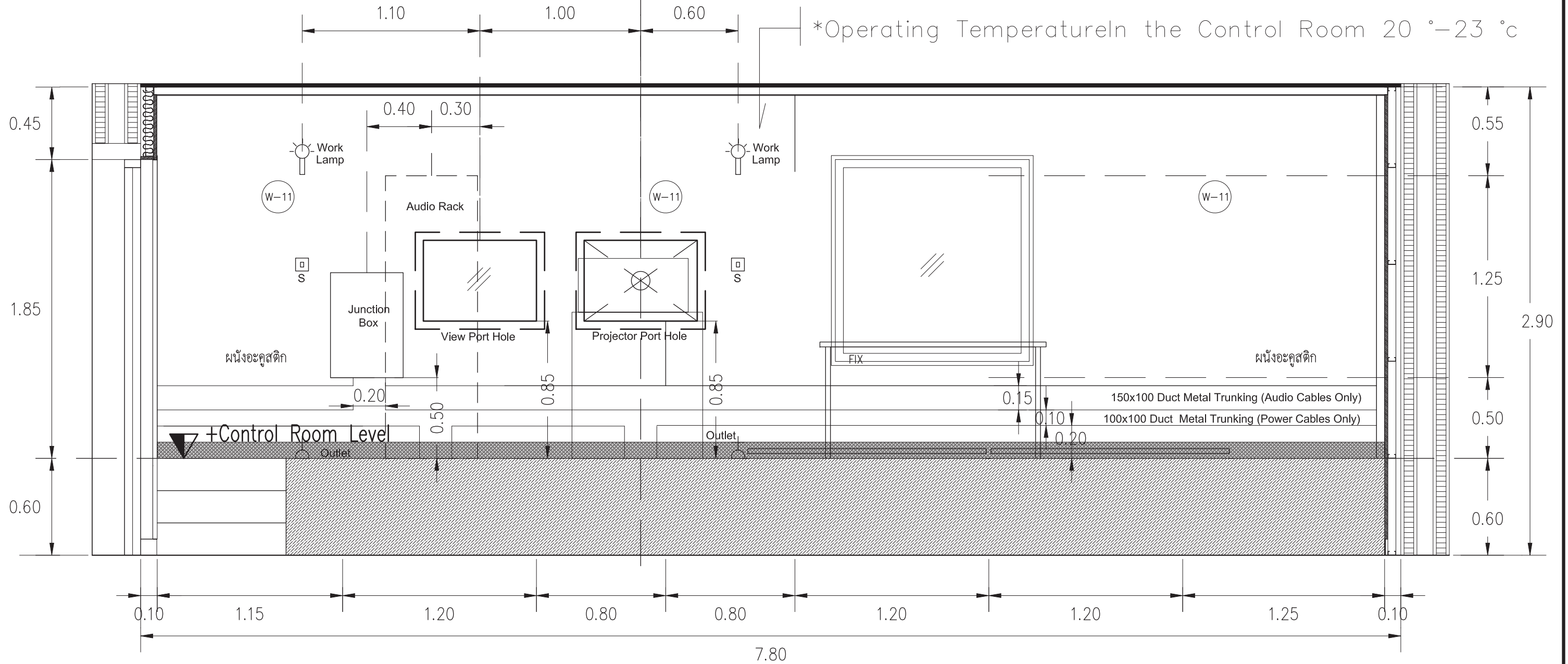
1 Detail Equipmaent Position Elevation for Control Room of Cosci Auditorium
