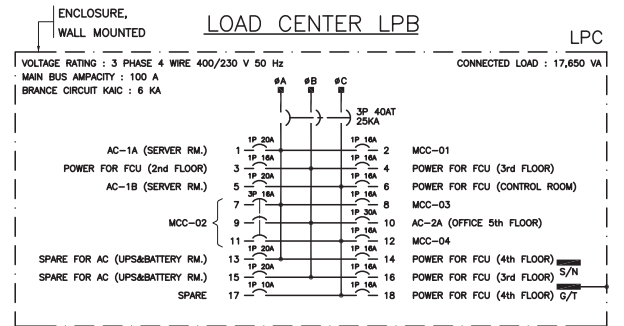
LOAD CENTER LPC
