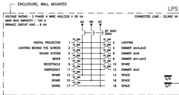
LOAD CENTER LPS
