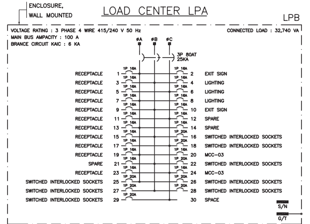
LOAD CENTER LPB
