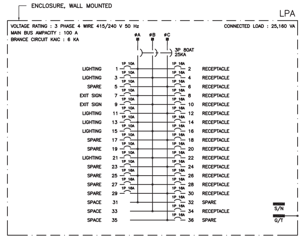
LOAD CENTER LPA
